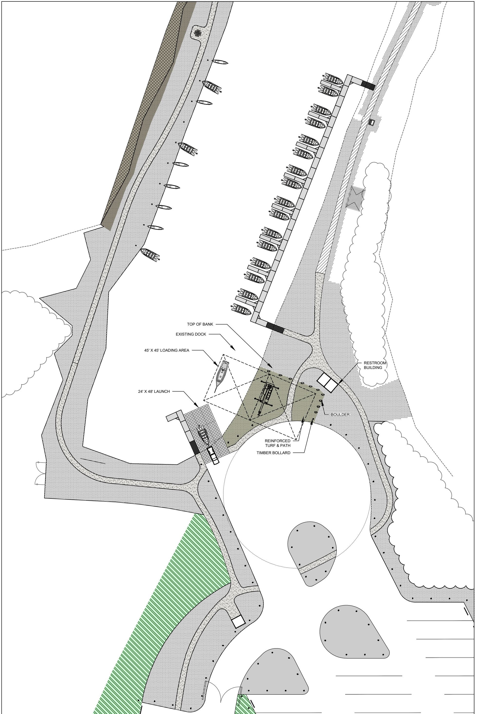
LAKE WABAMUN SUNDANCE BOAT DOCK LAUNCH - SAIL BOAT CONCEPT
