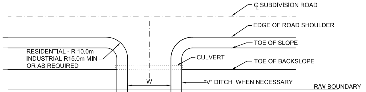
APPROACH PLAN
