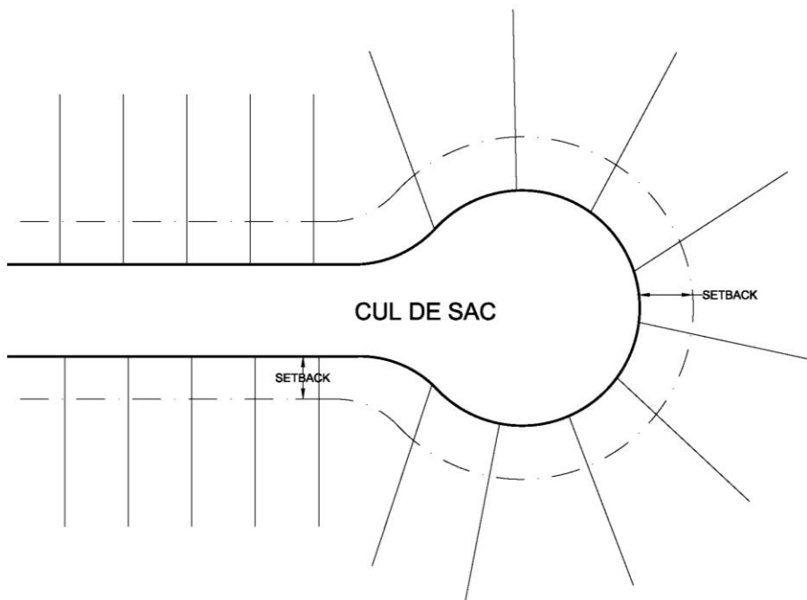
Figure 5: Setbacks
